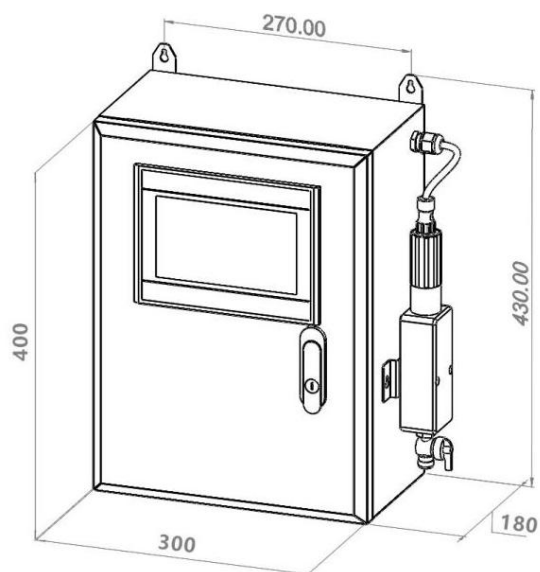
Fig.1 Protective box dimensions
