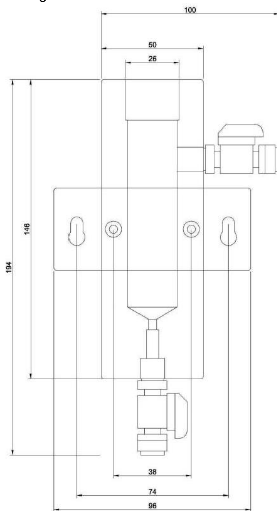
Fig.1 Protective box dimensions
